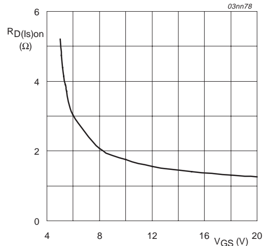
Fig 16. Drain- I_{\text{sense}} on-state resistance as function of gate-source voltage; typical values.
